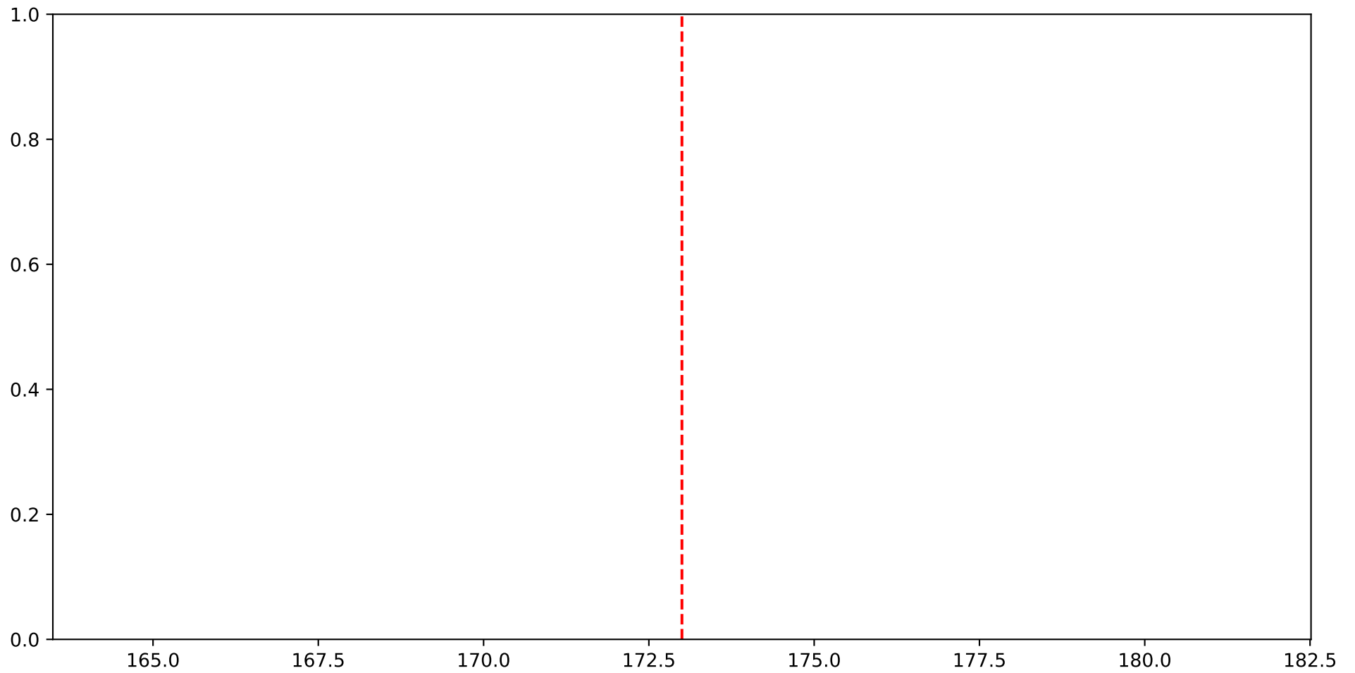
L1AC1 (plot by adjDAT)
