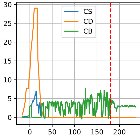
L1AC4: ['CS', 'CD', 'CB']
