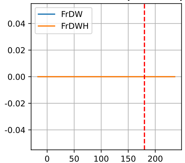
L1AC4: ['LfDW', 'FrDW', 'FrDWH'] L1AC4: ['FrDW', 'FrDWH', 'adjFrDW', 'adjFrDWH']
