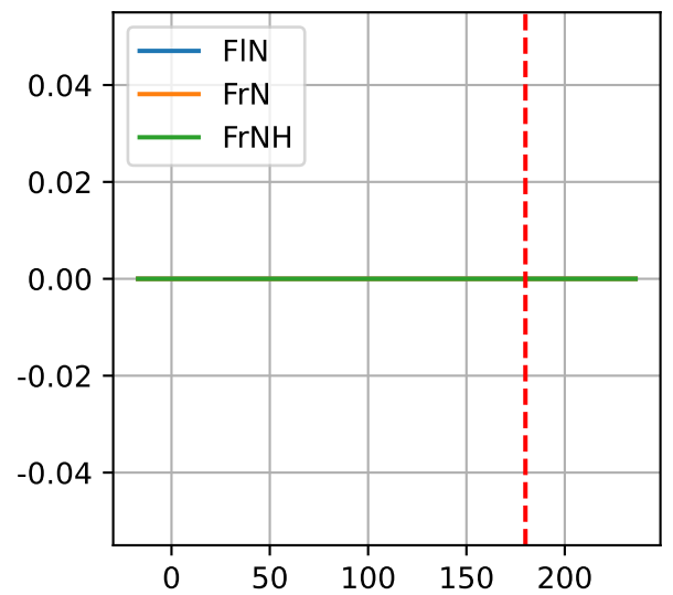
L1AC4: ['FIN', 'FrN', 'FrNH']
