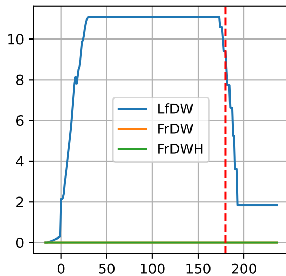
L1AC4: ['LfDW', 'FrDW', 'FrDWH'] L1AC4: ['FrDW', 'FrDWH', 'adjFrDW', 'adjFrDWH']
