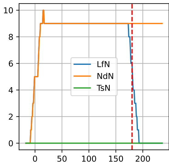
L1AC4: ['LfN', 'NdN', 'TsN']
