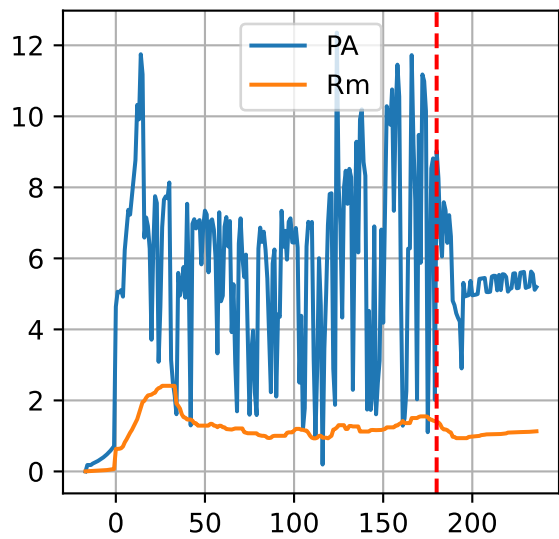
L1AC4: ['PA', 'Rm']
