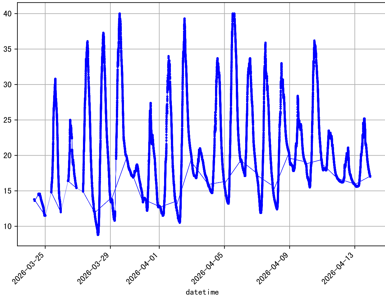
'Raw' data (20 days, 0 min/dp) 108941@122422IS_Ts_E14
