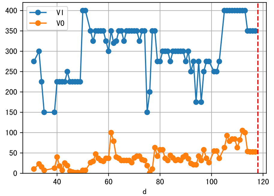
fgNum 2 (at_row = 32)
