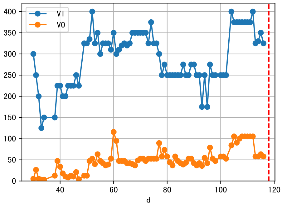
fgNum 1 (at_row = 3)
