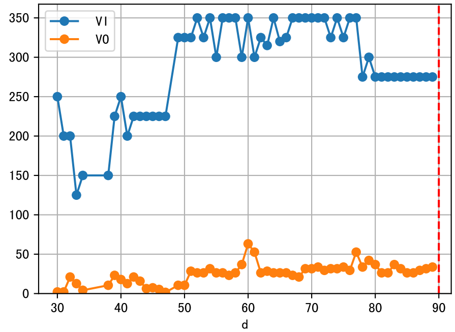
fgNum 2 (at_row = 35)
